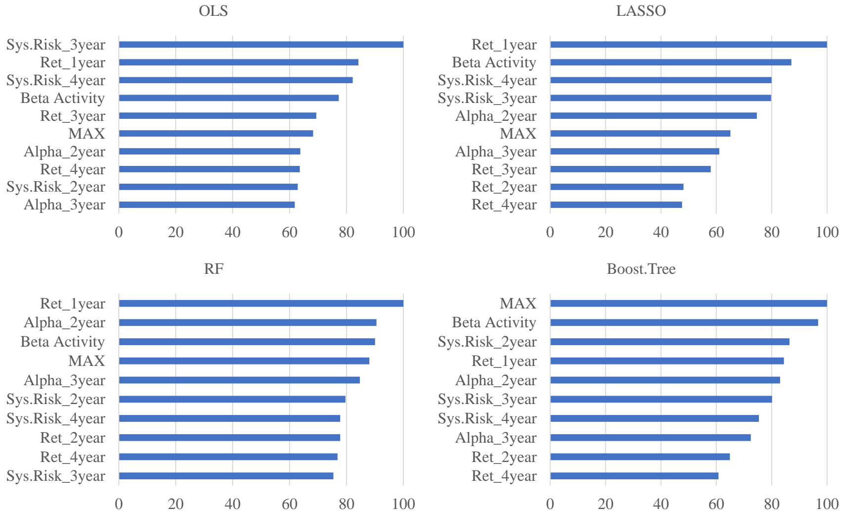
Figure 2.2: Predictor importance
